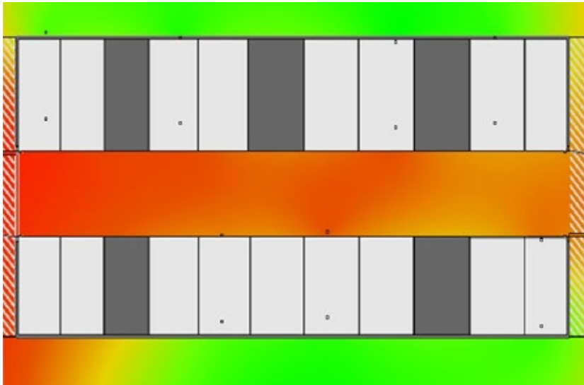
Above- A contained hot aisle of the high-density computing room prevents hot air from mixing with cool air, reducing the energy needed to air condition the room. This efficiency results in a PUE of 1.27.
